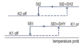
Figure 2: 2 INDEPENDENT STAGES WITH 1 PROBE if Sdb=0, Pr2=0 Example with Act=0 & Ac2=0
