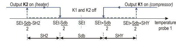
Figure 1: when Sdb > 0 DEAD BAND CONTROL is activated
