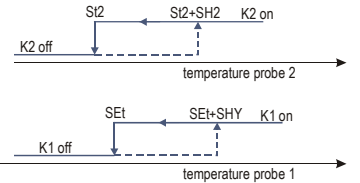
Figure 3: 2 INDEPENDENT STAGES WITH 2 PROBES if Sdb=0, Pr2=1 Example with Act=0 & Ac2=0
